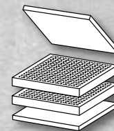
X2 LAYERS PLUCK FOAM Interior Dimensions: 13.5" L x 15.5" W x 4.25" D Exterior Dimensions: 15.75" L x 12" W x 3.125" H
